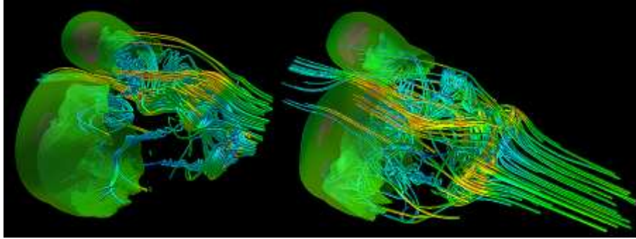
Fig. 2. Initial compression in SW/MCs interaction ( t = 40, 60 ).
